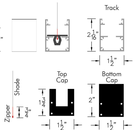
U Channel (Inside Mount)
