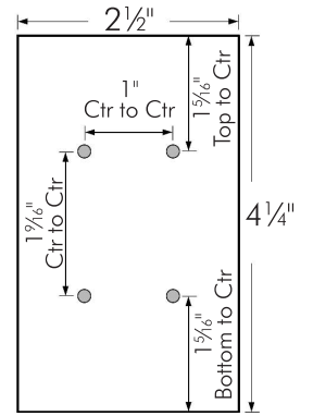
Wall Bracket for Cassette Box
